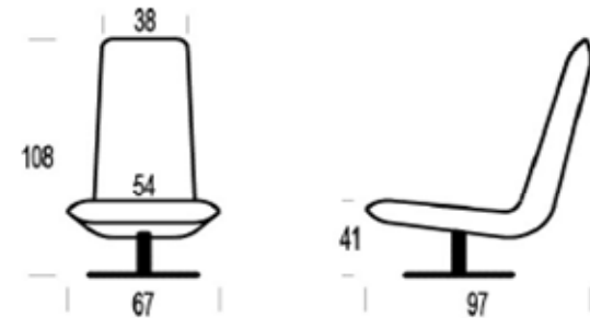
el.18 - 18A
